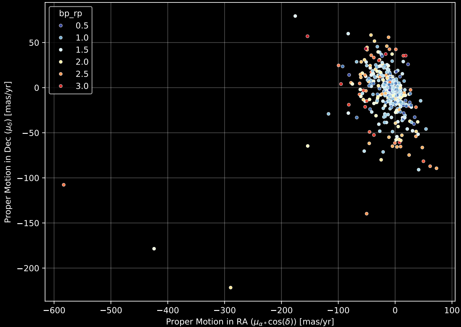
APOGEE DR17 Field: [090+60] Proper Motion Diagram (n= 469)
