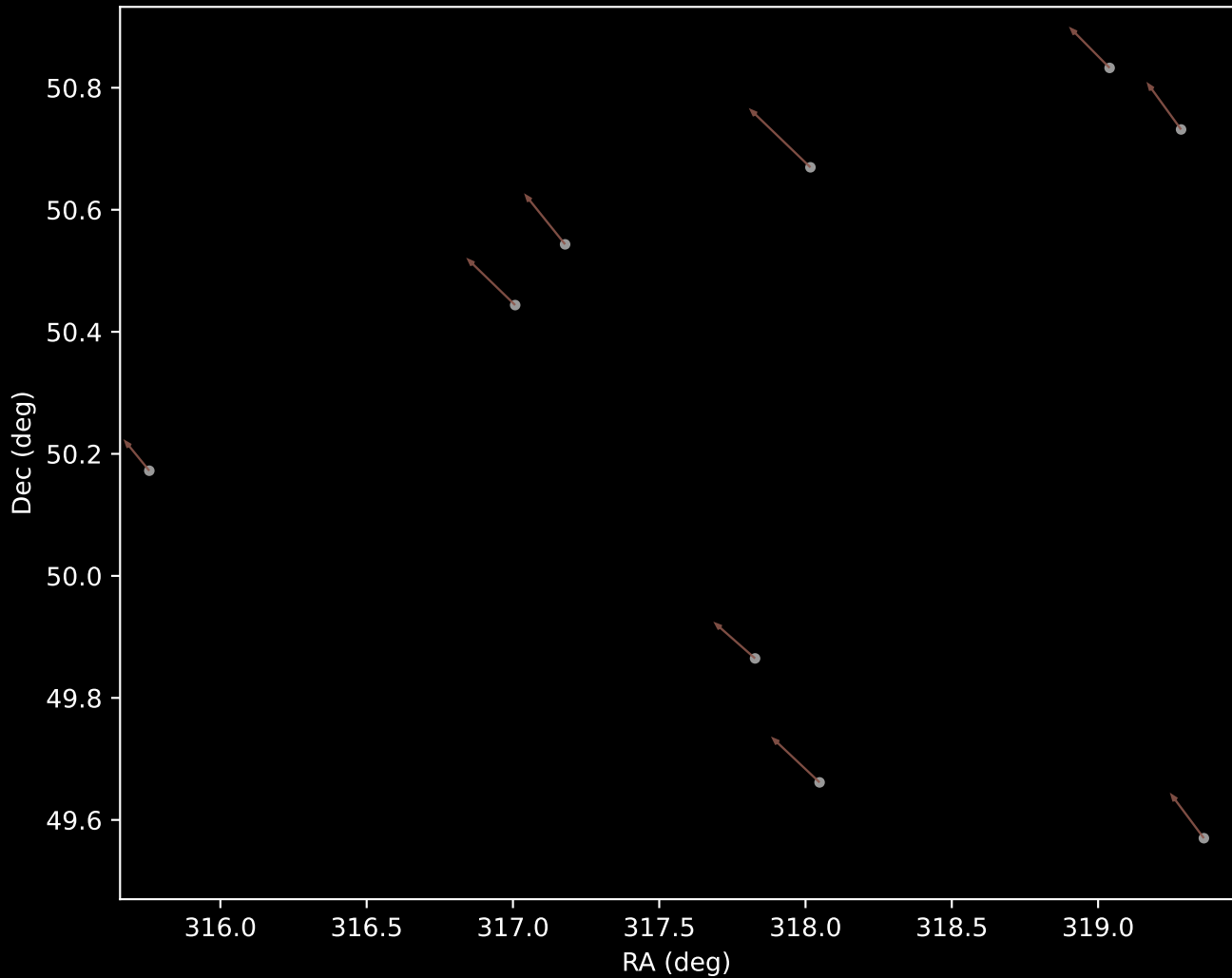
APOGEE DR17 Cluster 10 Proper Motion Vectors (n=9)
