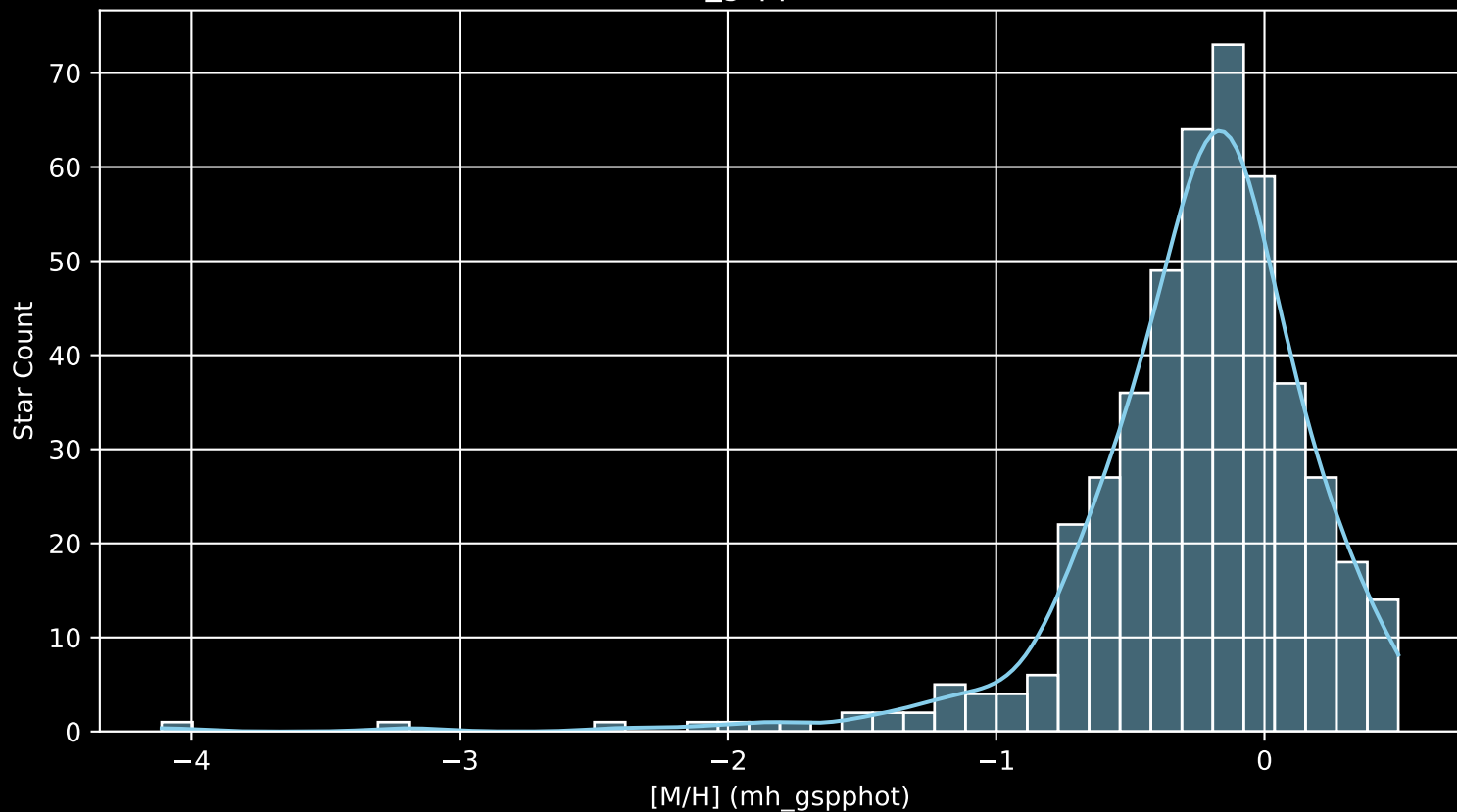
APOGEE DR17 Field: [090+60 [M/H] (mh_gspphot) (n= 458)
