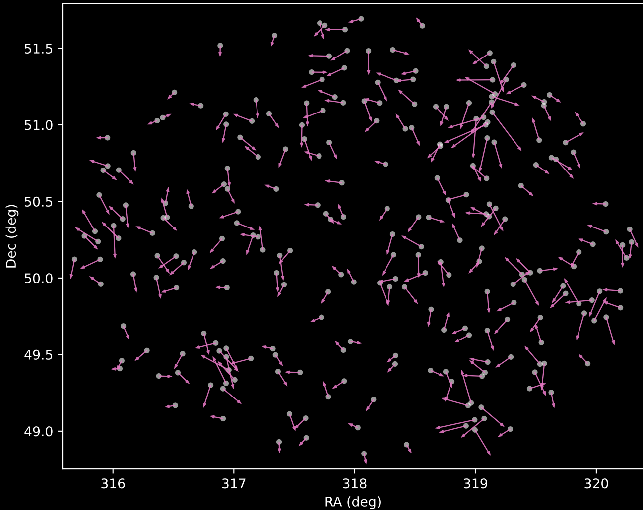
APOGEE DR17 Cluster 12 Proper Motion Vectors (n=251)
