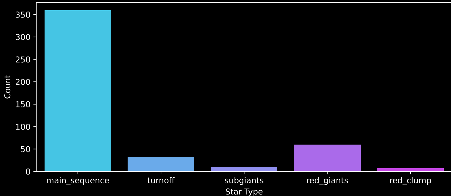
APOGEE DR17 Field: [090+60] Count plot of Star Type
