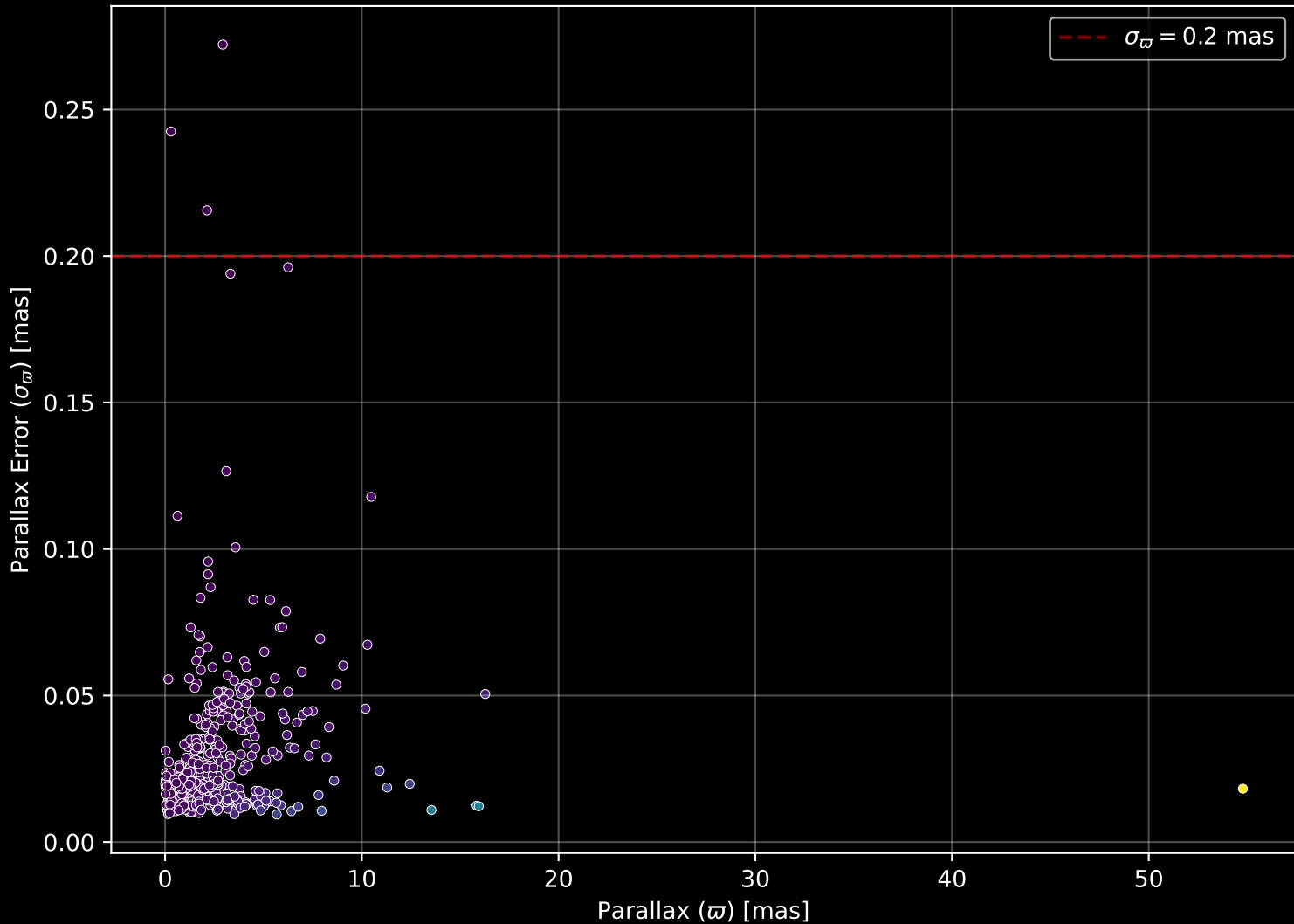
APOGEE DR17 Field: [090+60] Parallax Quality (n= 469)
