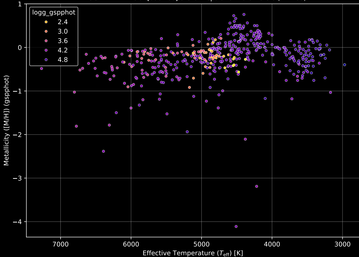
APOGEE DR17 Field: [090+60] Stellar Population Parameters (n= 469)
