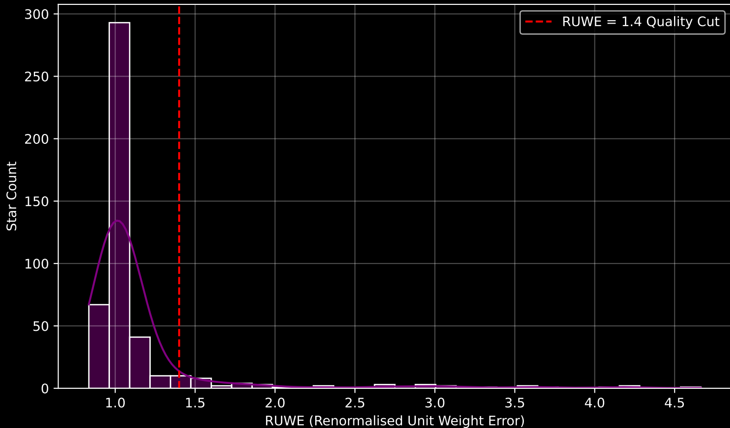
GAPOGEE DR17 Field [090+60] RUWE Distribution (n= 457)
